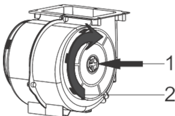
Fig. 6: Carbon Filter
